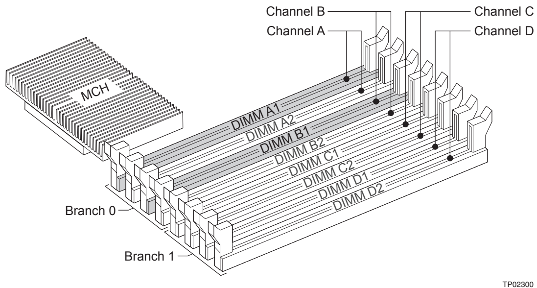
Figure 12. Recommended Minimum Two DIMM Memory Configuration
