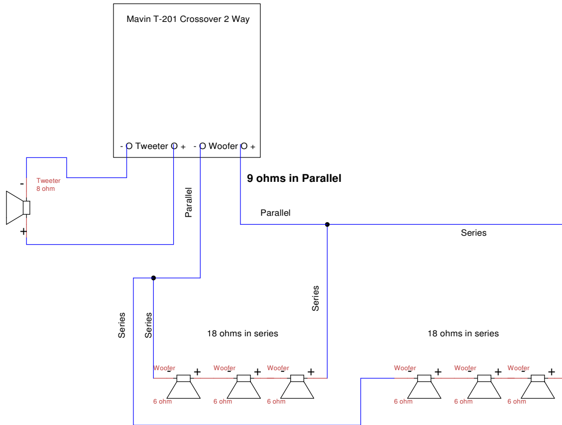
Mavin 6.5" Six Pack Bass Driver times 6 Series Parallel Wiring Configuration
