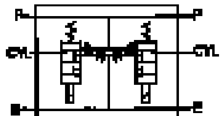
Four-Way Normally Open- Normally Open
